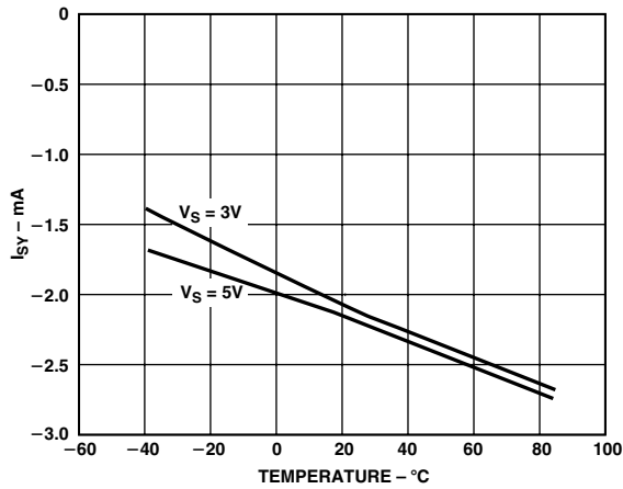
Figure 14. I_{SV-} vs. Temperature
