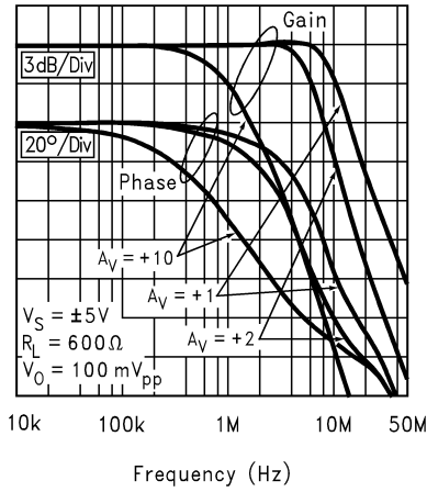
Closed Loop Frequency Response for Various Gains
