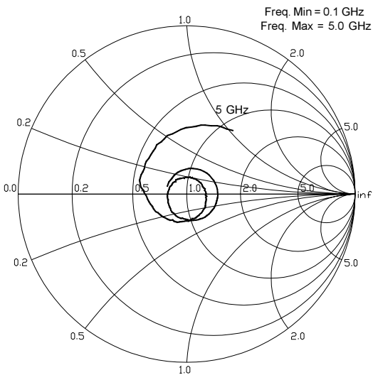
S11, I_D = 45\text{mA} , T_a = 25\text{C}
