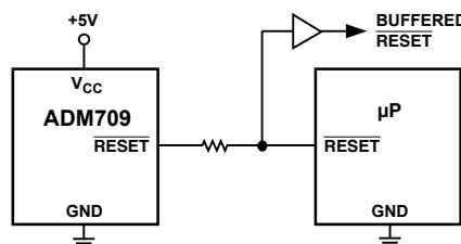
Figure 6. Interfacing to Microprocessors with Bidirectional RESET
