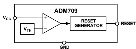
Figure 1. Functional Block Diagram
